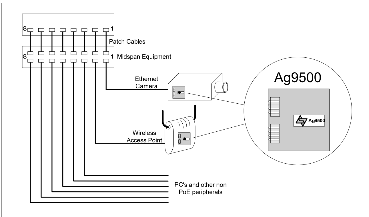
Figure 5: Typical Application
