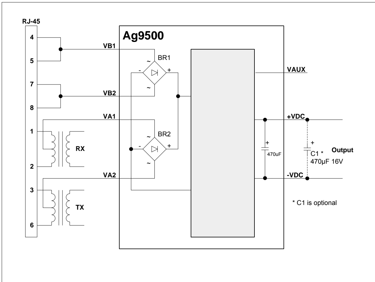
Figure 4: Typical Connection Diagram
