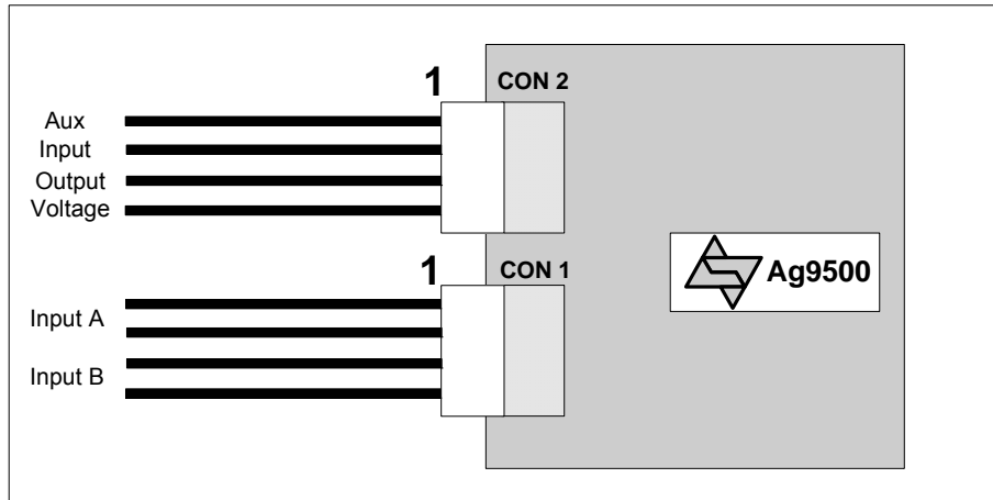
Figure 6: Typical Connection
